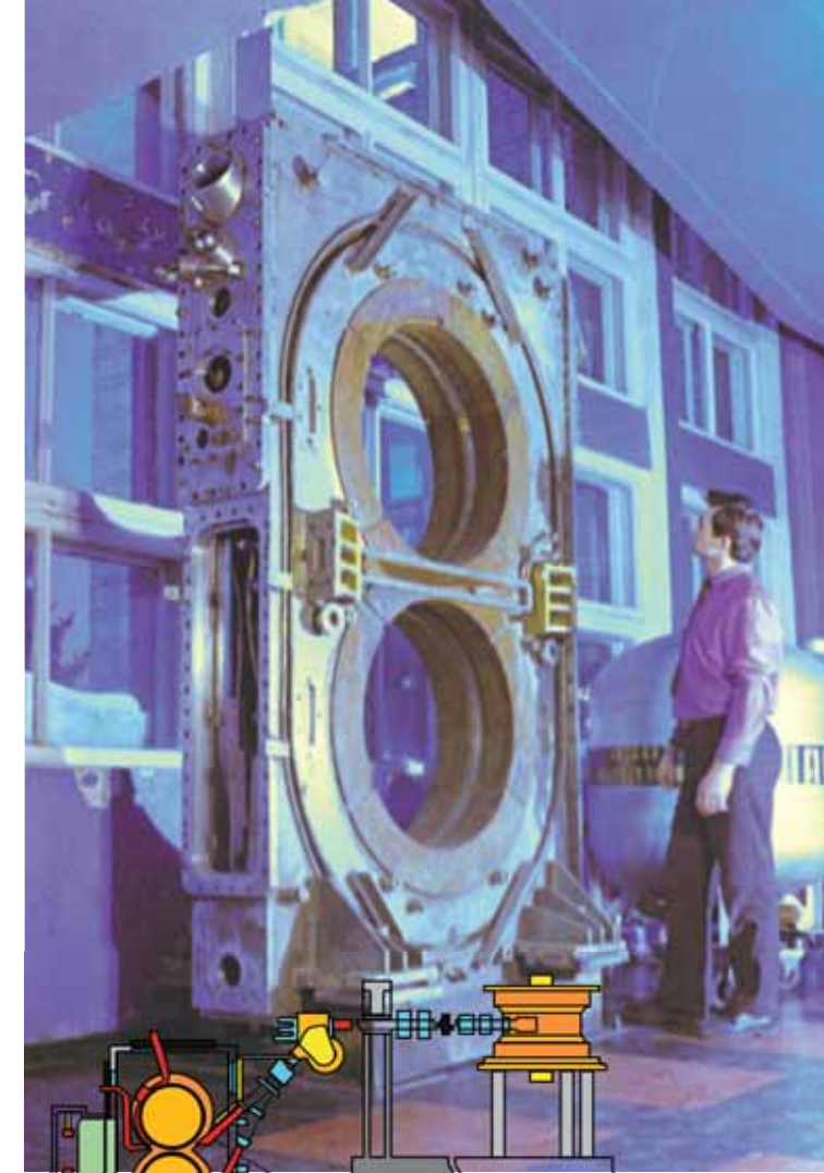
VEP-1 — first experimental setup of INP SB RAS with colliding electron beams with an energy of 2x160 MeV
