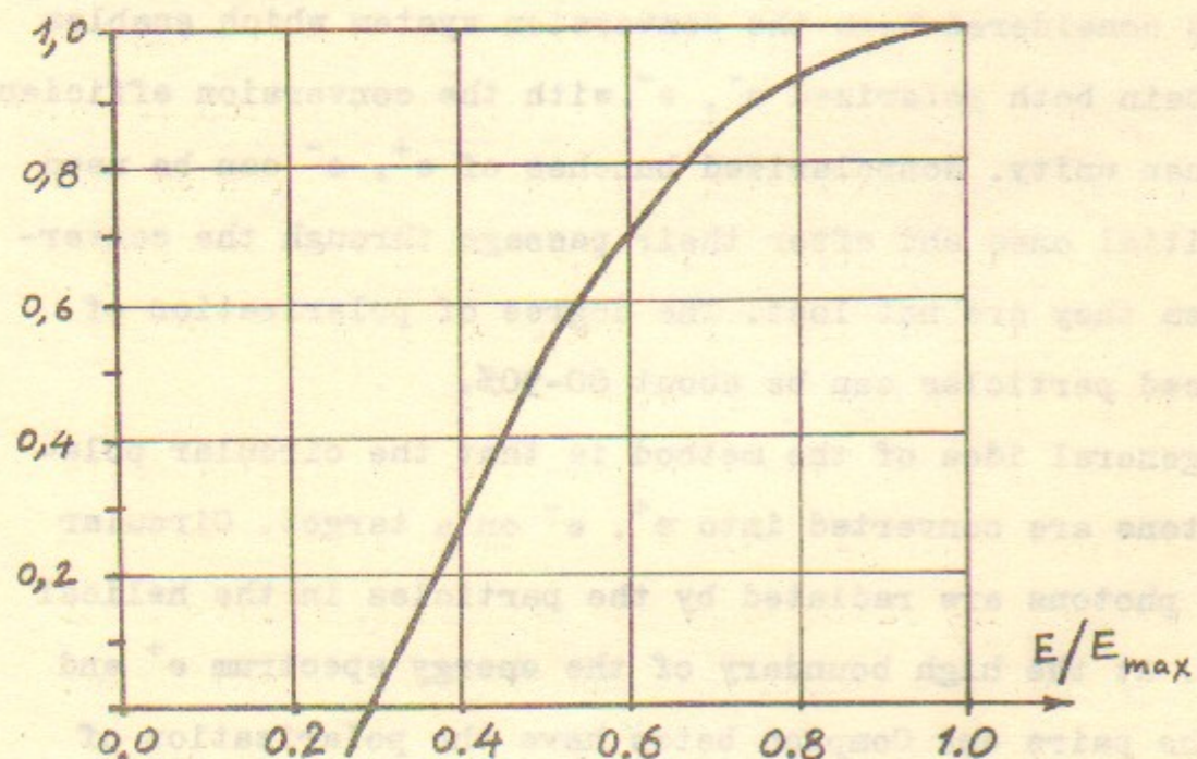
Fig.1 The longitudinal electron or positron polarization as a function of its energy /1/.
