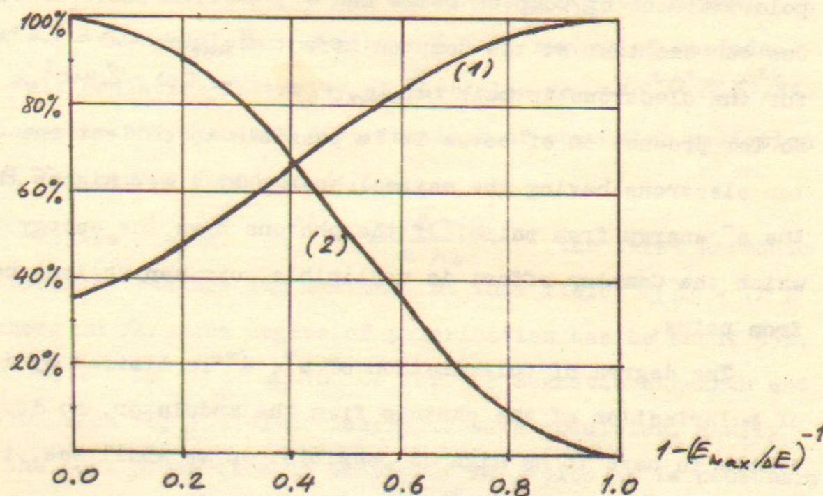
Fig.3 The mean polarization (1) and percentage of particles (2) as a function of the energy interval from the maximum particle energy.
